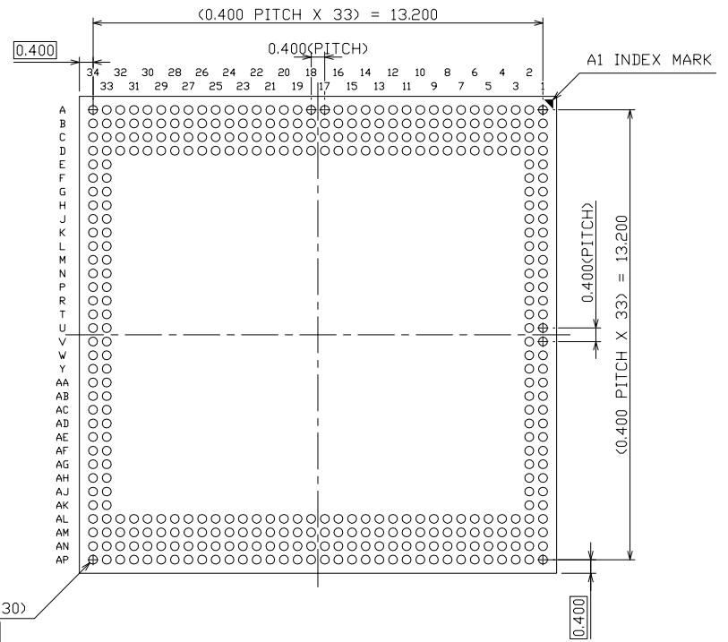
BOTTOM VIEW
