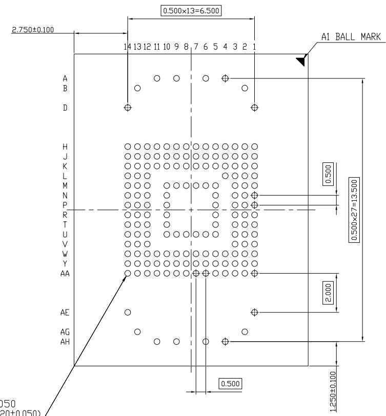
BOTTOM VIEW
