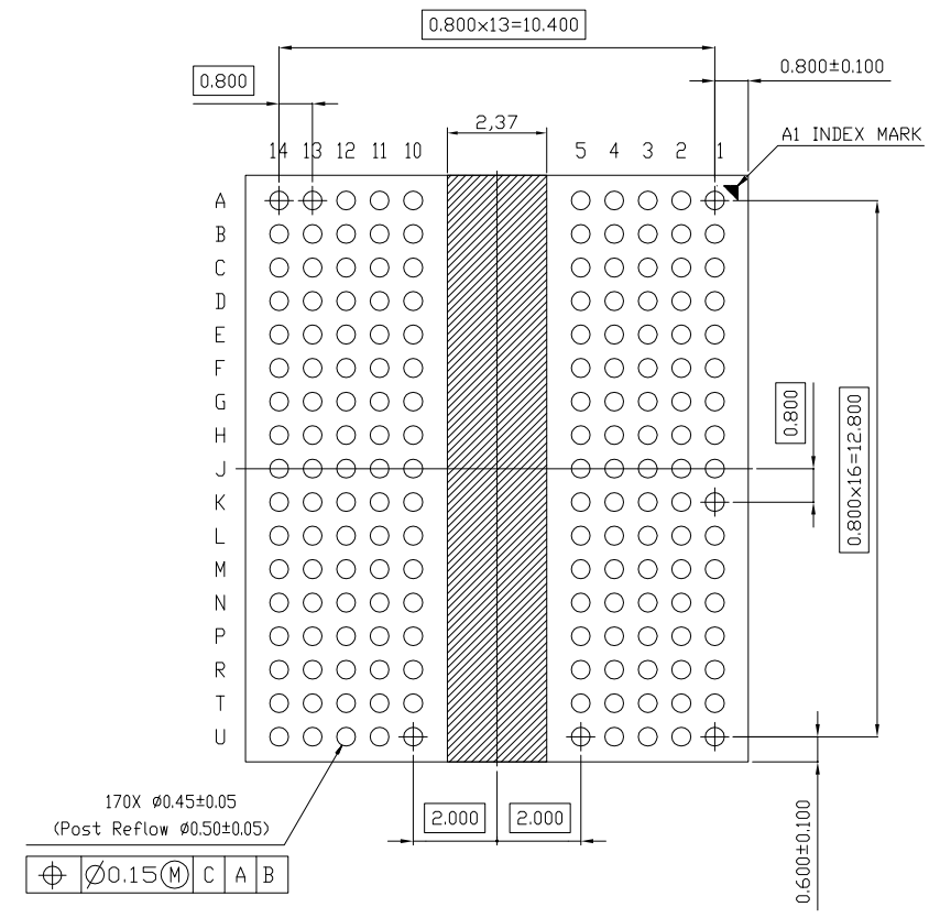
BOTTOM VIEW
