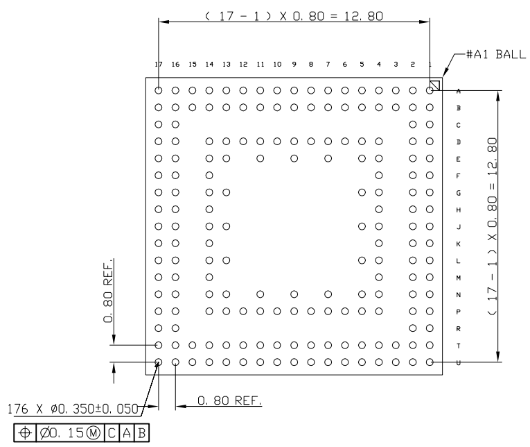
BOTTOM VIEW
