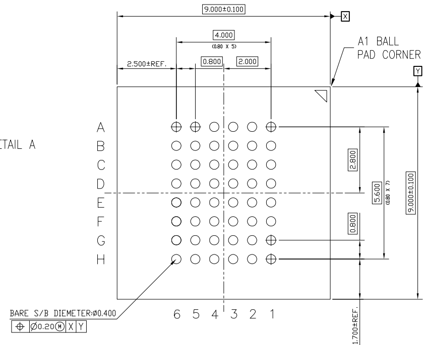
BOTTOM VIEW
